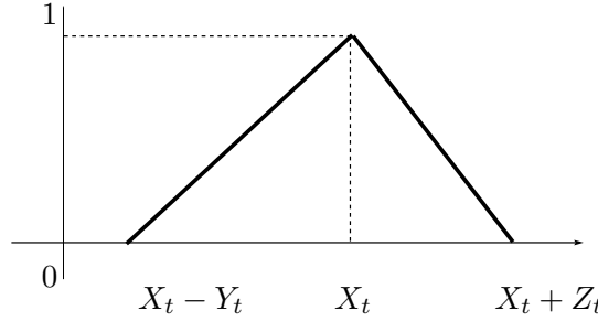
Figure 1. The fuzzy perception \tilde{X}_t = (Y_t, X_t, Z_t)
