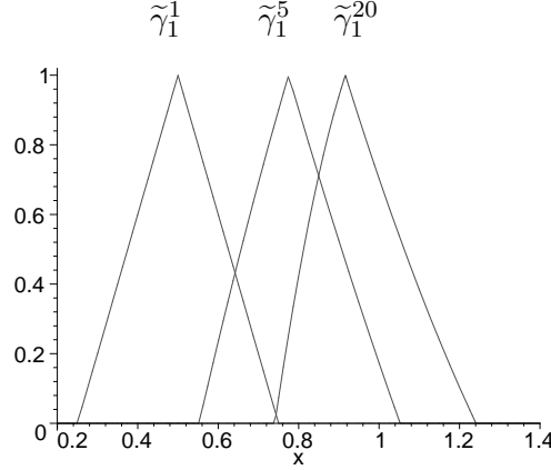
Figure 2. The graph of \tilde{\gamma}_1^n ( n = 1, 5, 20 )
