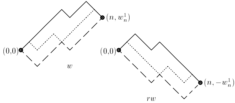
Figure 3: Examples of w and rw .
