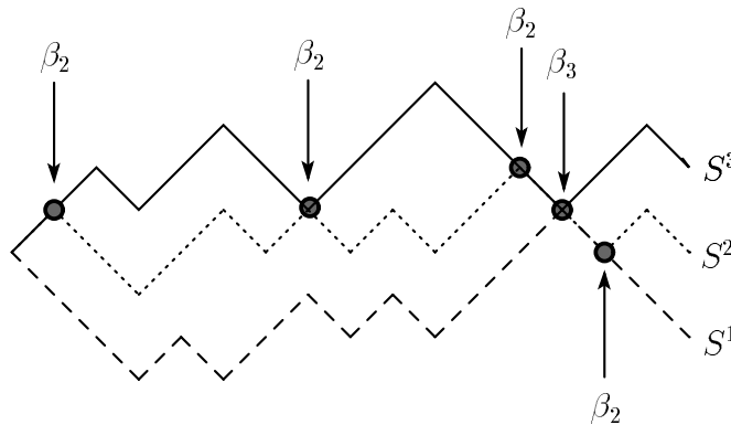
Figure 1: An example of 3-friendly walkers.
