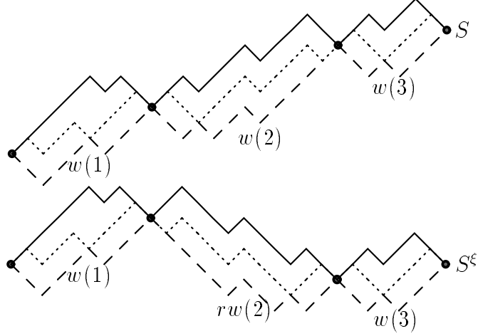
Figure 4: Examples of S and S^\xi , in the case that \tau_n = 3 , \xi_1 = 1 , \xi_2 = -1 and \xi_3 = 1 .
