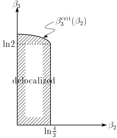
Figure 2: The delocalized phase for 3-friendly walkers.
